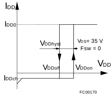
Figure 7. Shutdown Action
